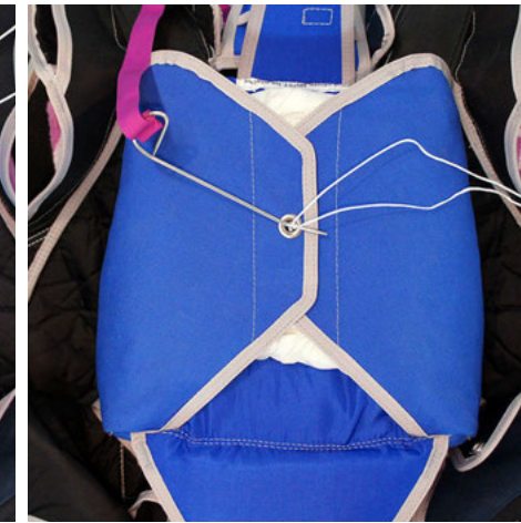
23. Close the left flap (#4).
