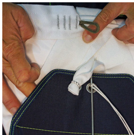
20. Tuck reserve bridle under the #1 flap.
